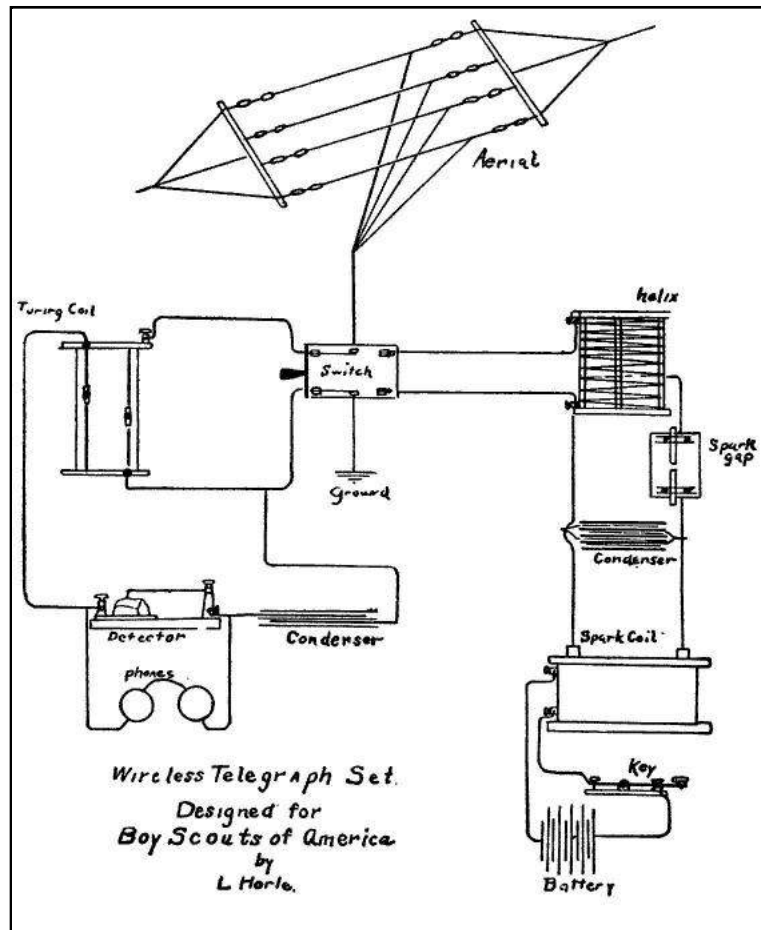
Wireless Telegraph Set Designed for Boy Scouts of America by L. Horle.
