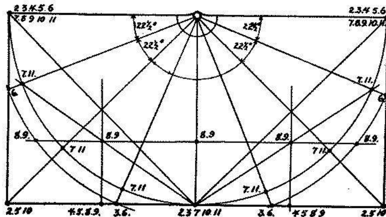
Fig. 12. Showing how ten different tents can be made with but one piece of canvas
