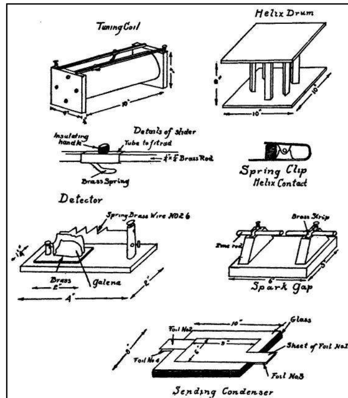
Details of instruments for field use.
