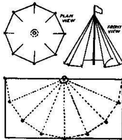
Fig. 7. Conical tent, or wigwam
